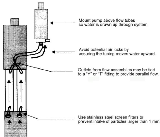
Figure 2. Proper connection of ac-s flow tube
