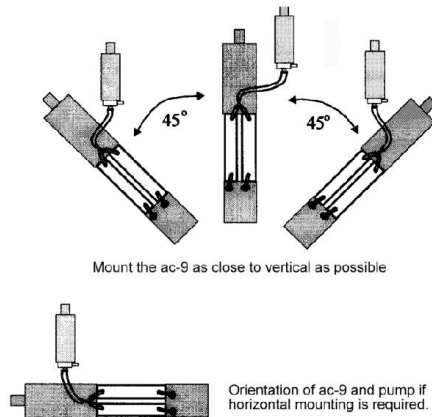
Figure 1. ac-s mounting positions
